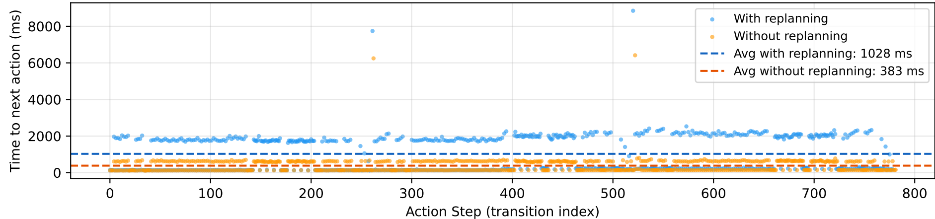
Time Delta Between Consecutive ML Actions
